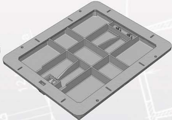
Cover Set - Viewed From Underneath
